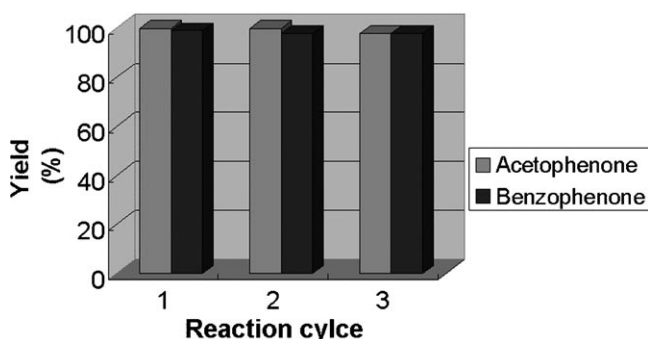
Figure 2. Reusability of Sn-Mont for the cyanosilylation of acetophenone and benzophenone, respectively.
