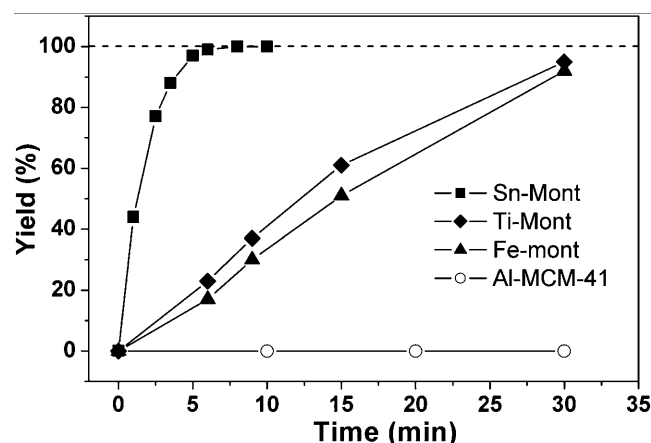
Figure 1. Time-course of the cyanosilylation of benzophenone using Sn-Mont and control heterogeneous catalysts. Reaction conditions: benzophenone (1 mmol); TMSCN (1.2 mmol); \text{CH}_2\text{Cl}_2 (2 mL); catalyst (10 mg); room temperature.
